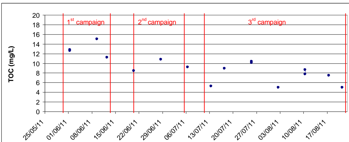
Figure 15 Total organic carbon in water samples.
