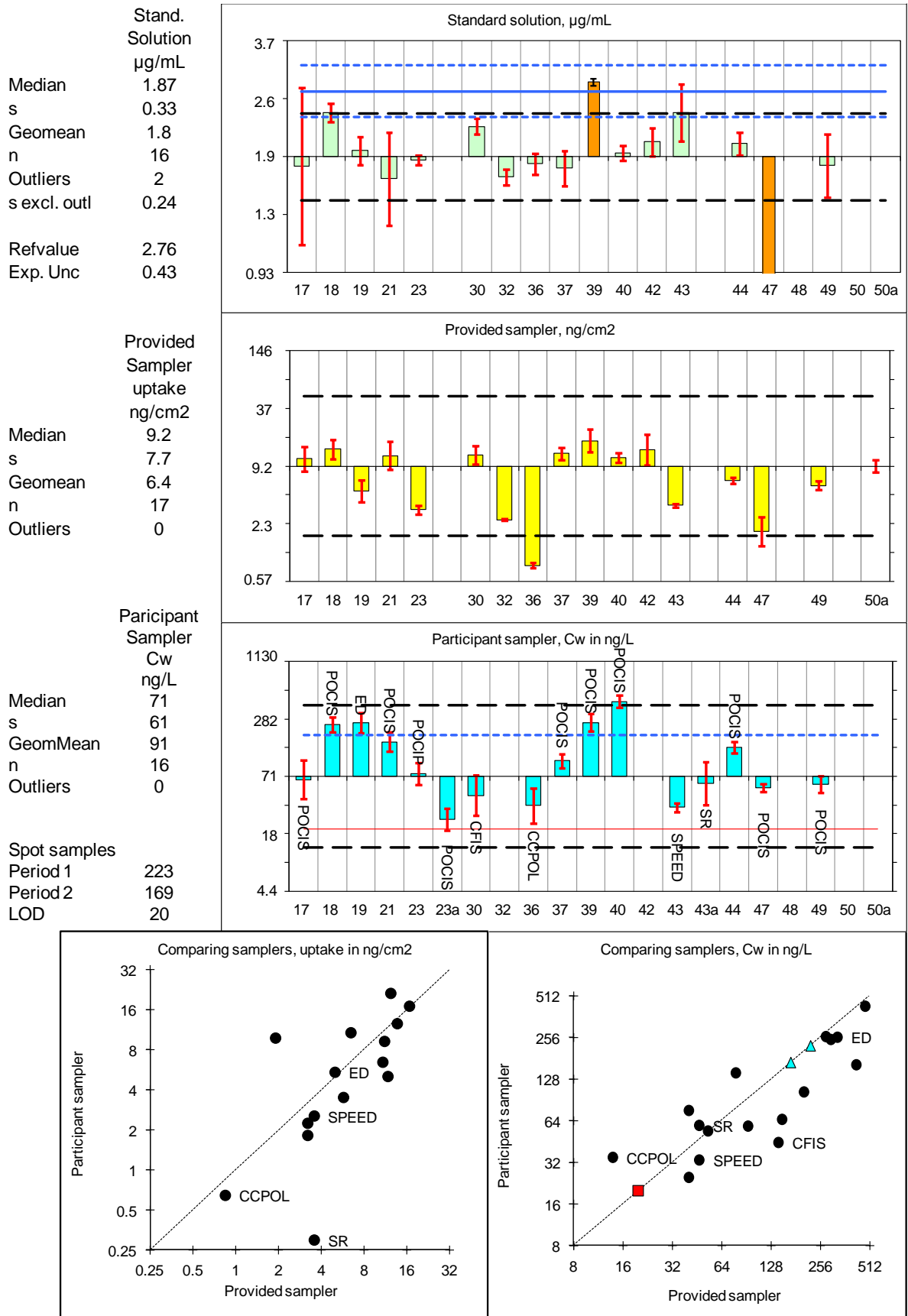
Figure 24 Results of analysis of diuron. Graph explanation is given in 10.2. and 10.3
