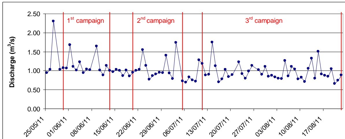
Figure 10 Water discharge.
