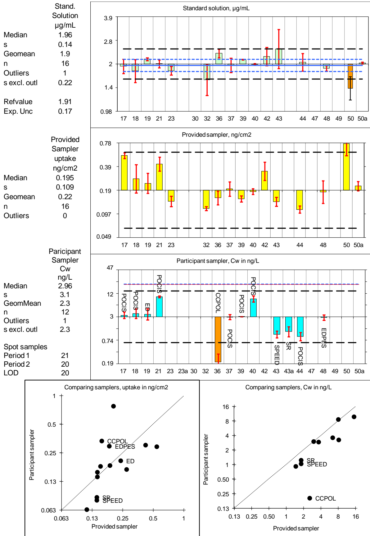
Figure 25 Results of analysis of S-metolachlor. Graph explanation is given in 10.2.and 10.3
