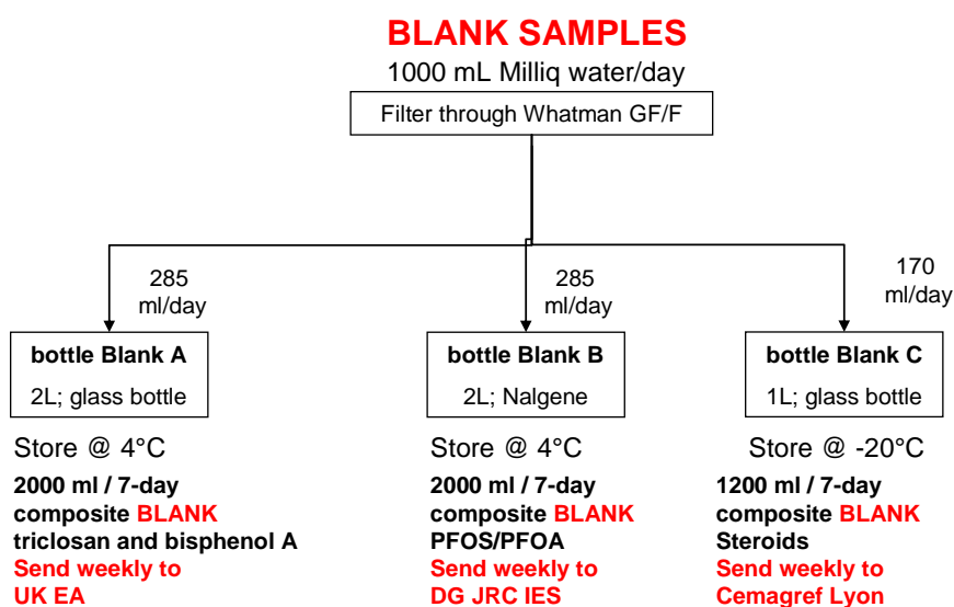
Figure 17 Water sampling scheme for obtaining 7-day composite water samples for analysis of triclosan, bisphenol A, PFOS, PFOA and steroid hormones.
