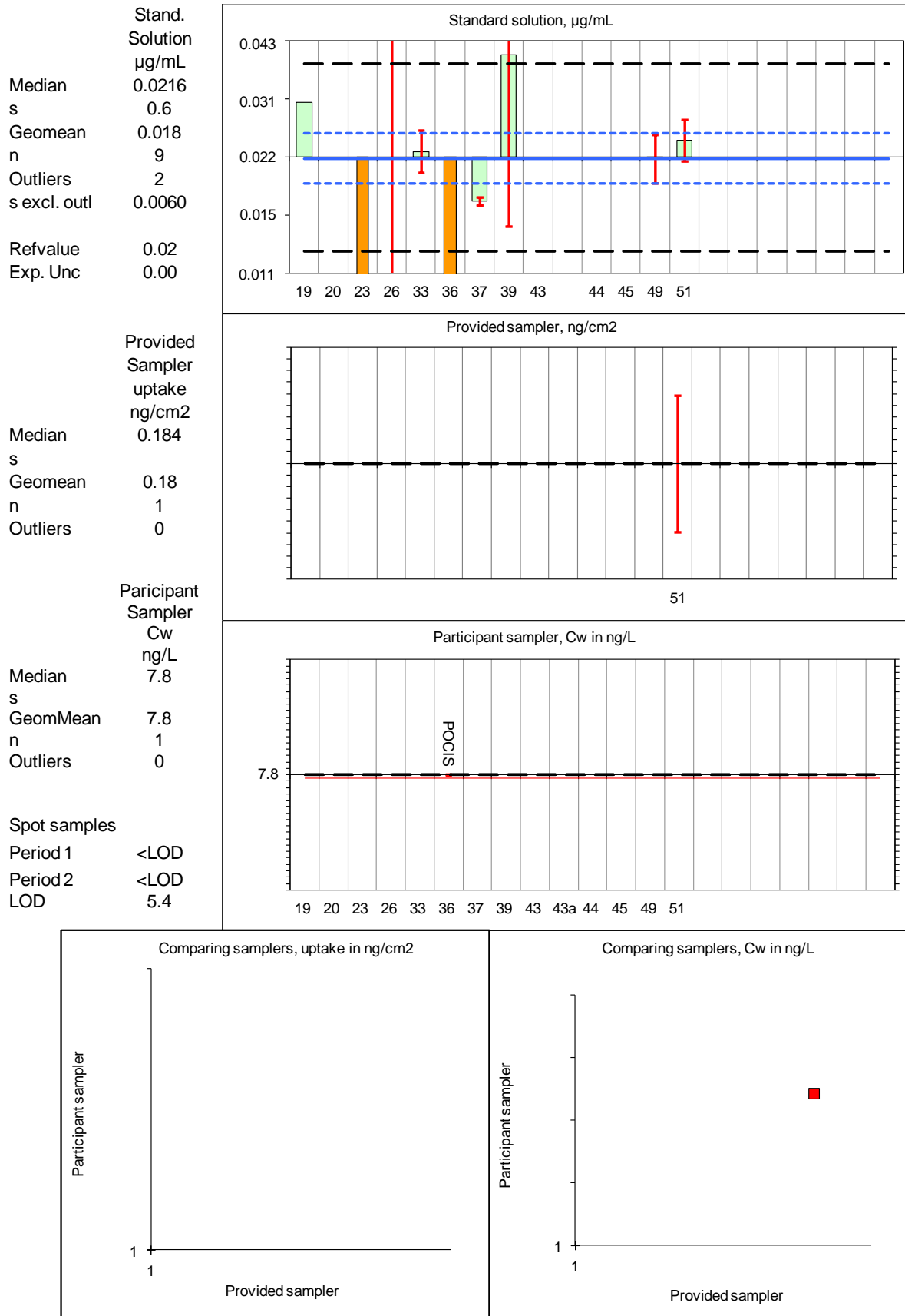
Figure 44 Results of analysis of estriol. Graph explanation is given in 10.2.and 10.3.
