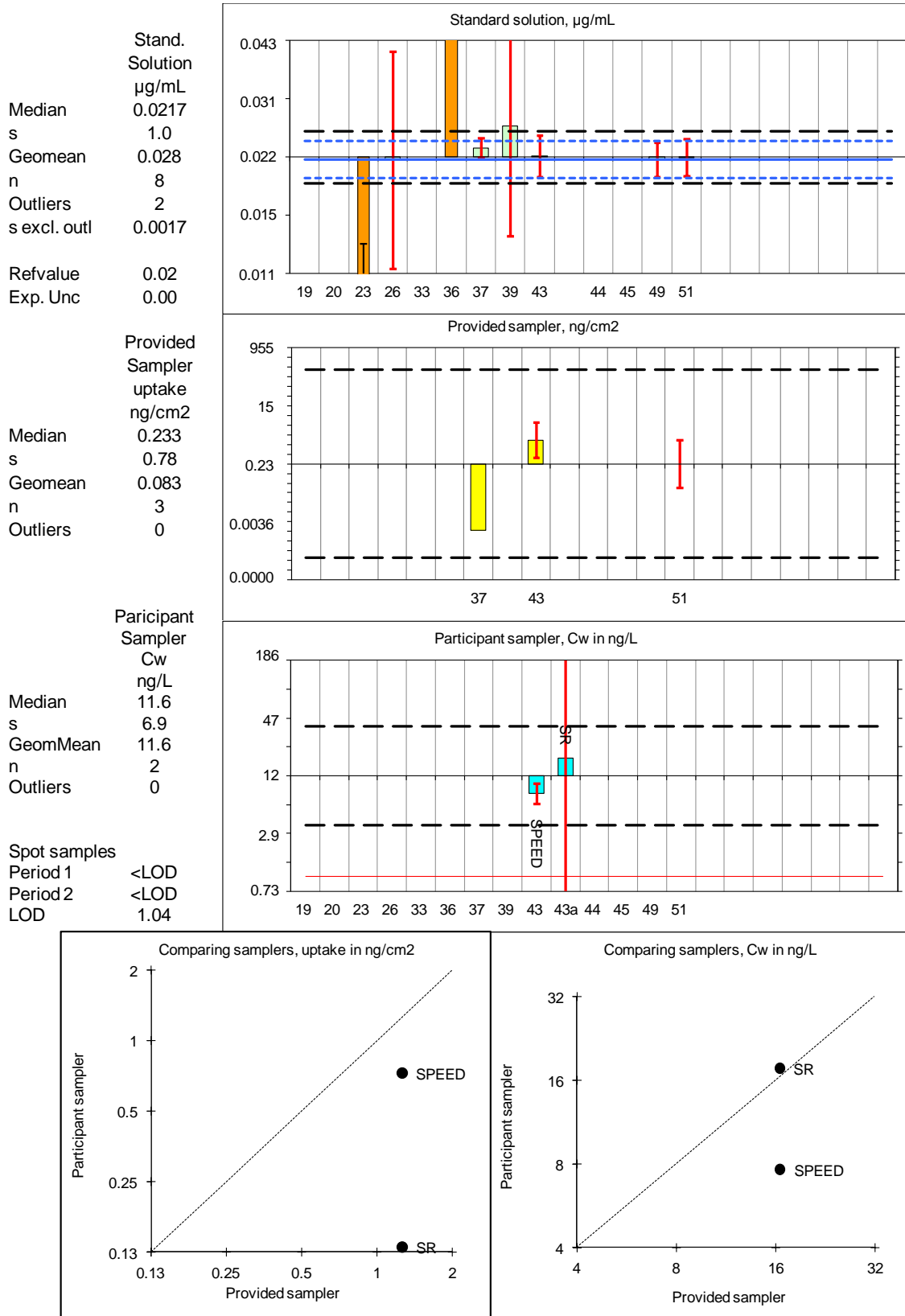
Figure 41 Results of analysis of 17-alpha-estradiol. Graph explanation is given in 10.2.and 10.3.
